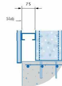
Section Thru B GUTTER SIDE WALL No Rebate
