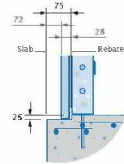
Section Thru A GABLE END 25mm Deep Rebate
